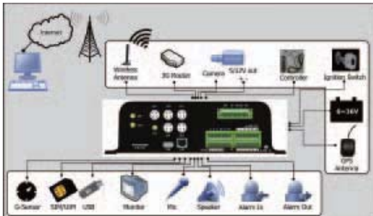
Rear Panel of DS-8104HMI-A
